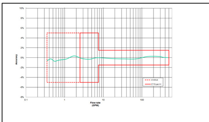
Accuracy curve (3")
